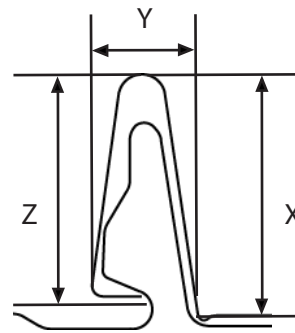
1" - 1 1/2" Snap Lock
