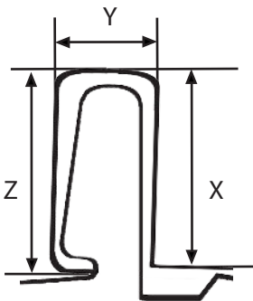
1" - 1 1/2" Snap Lock
