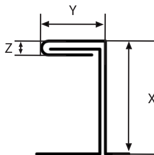
Single Lock "L"
