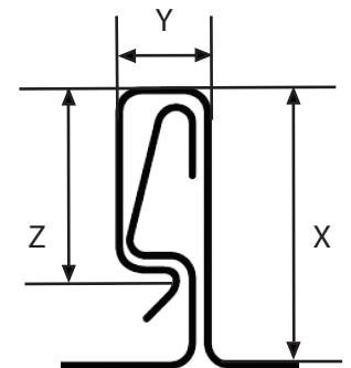
1" - 1 1/2" Snap Lock
