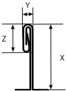
Double Lock
