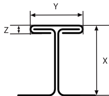
Tee Seam
