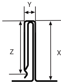
1 3/4" Snap Lock
