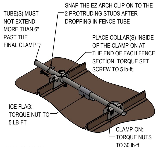
1" TO 1-1/2" SNAPLOCK
