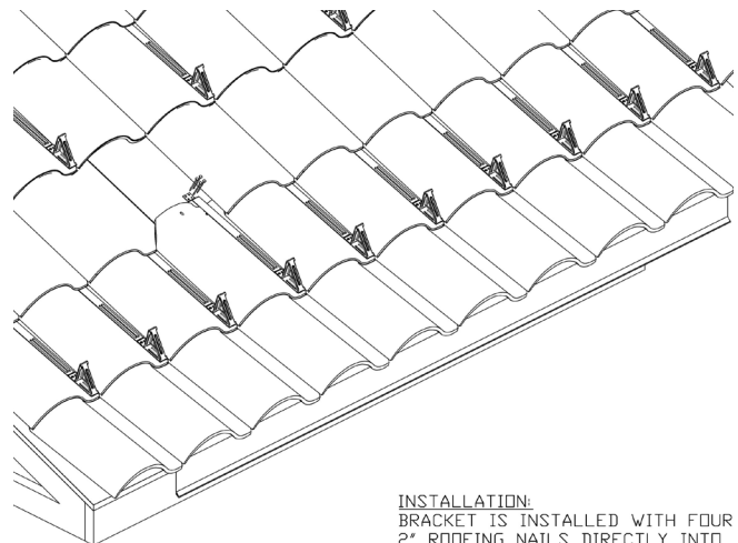
SNOW BRACKET 'LUDOWICI HIGH PROFILE' TILE ROOF
