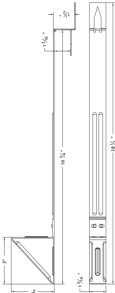
DIMENSIONS *Dimensions shown are in inches. DO NOT SCALE
